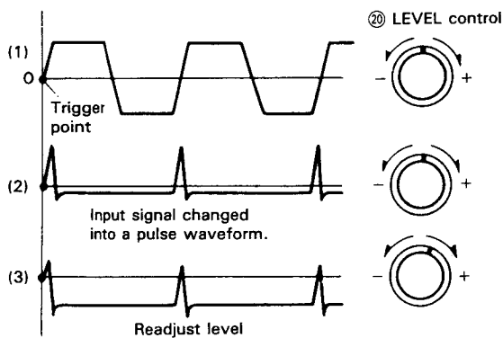
(a) When the trigger level is set around the center of the waveform.
